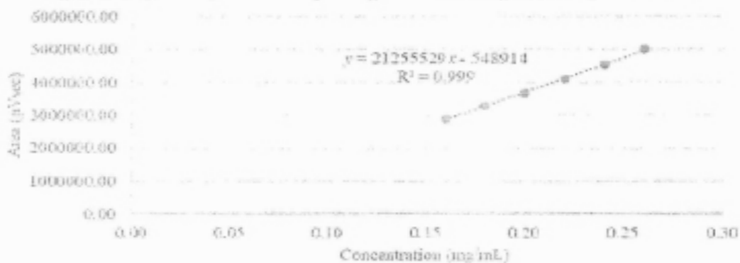
Figure 1. Graphical representation of the regression line using the least squared method
